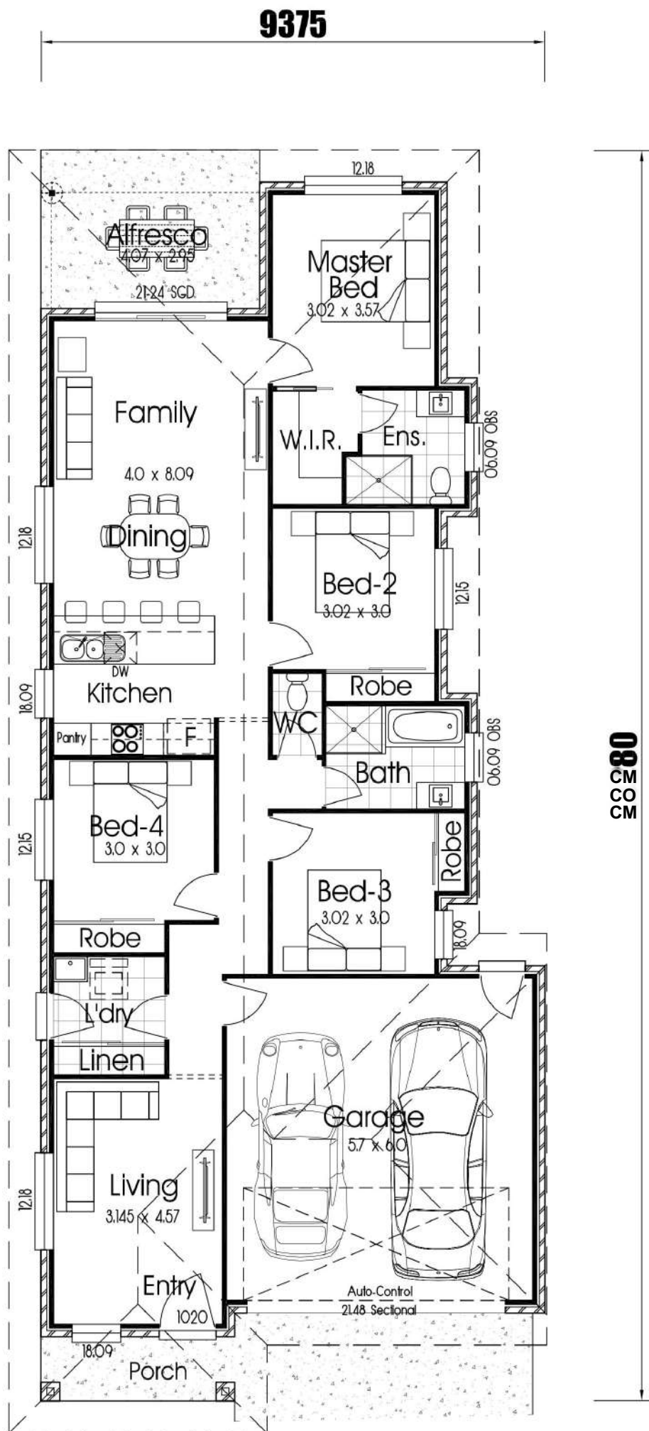
Floor Plan
